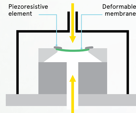
Figure 7: Piezoresistive sensor
